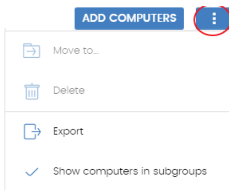
Figure 3.8: Context menus
