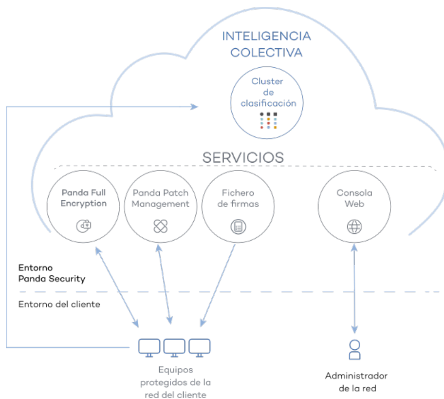
Figure 2.3: Panda Endpoint Protection general structure
