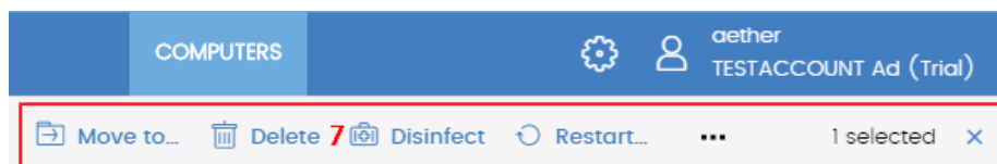
Figure 8.6: Action bar
