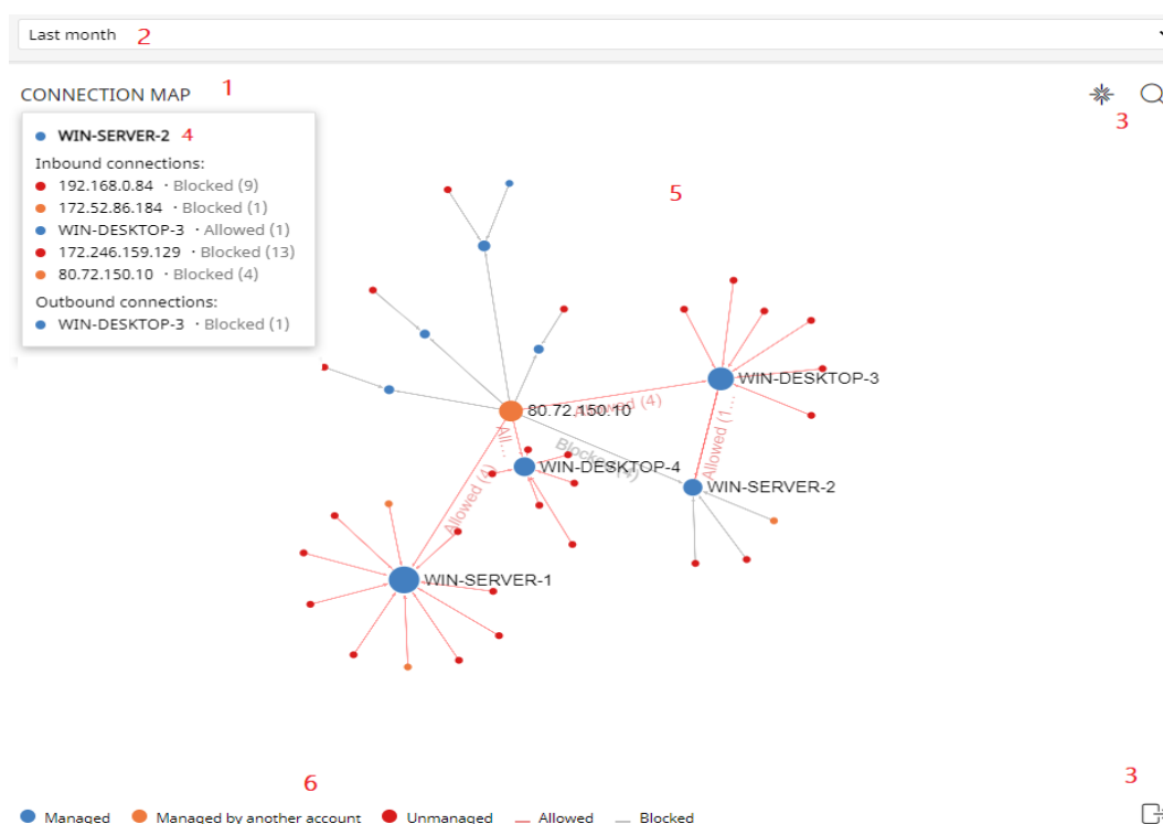
Figure 14.20: Connection Map
