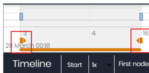
Figure 23.2: Time selectors
