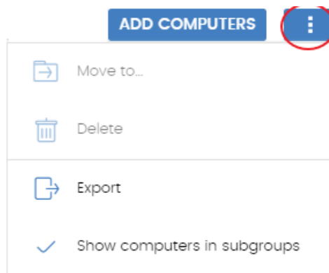
Figure 3.8: Context menus
